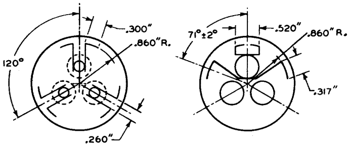
LOCATION OF RADIAL- CONVERGING POLE PIECES
