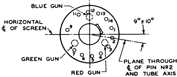
BASE BOTTOM VIEW
