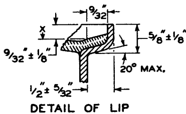
DETAIL OF LIP
