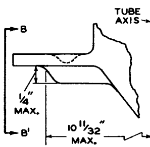
EXTERNAL VIEW AT A-A' DETAIL OF FLANGE BOSSES
